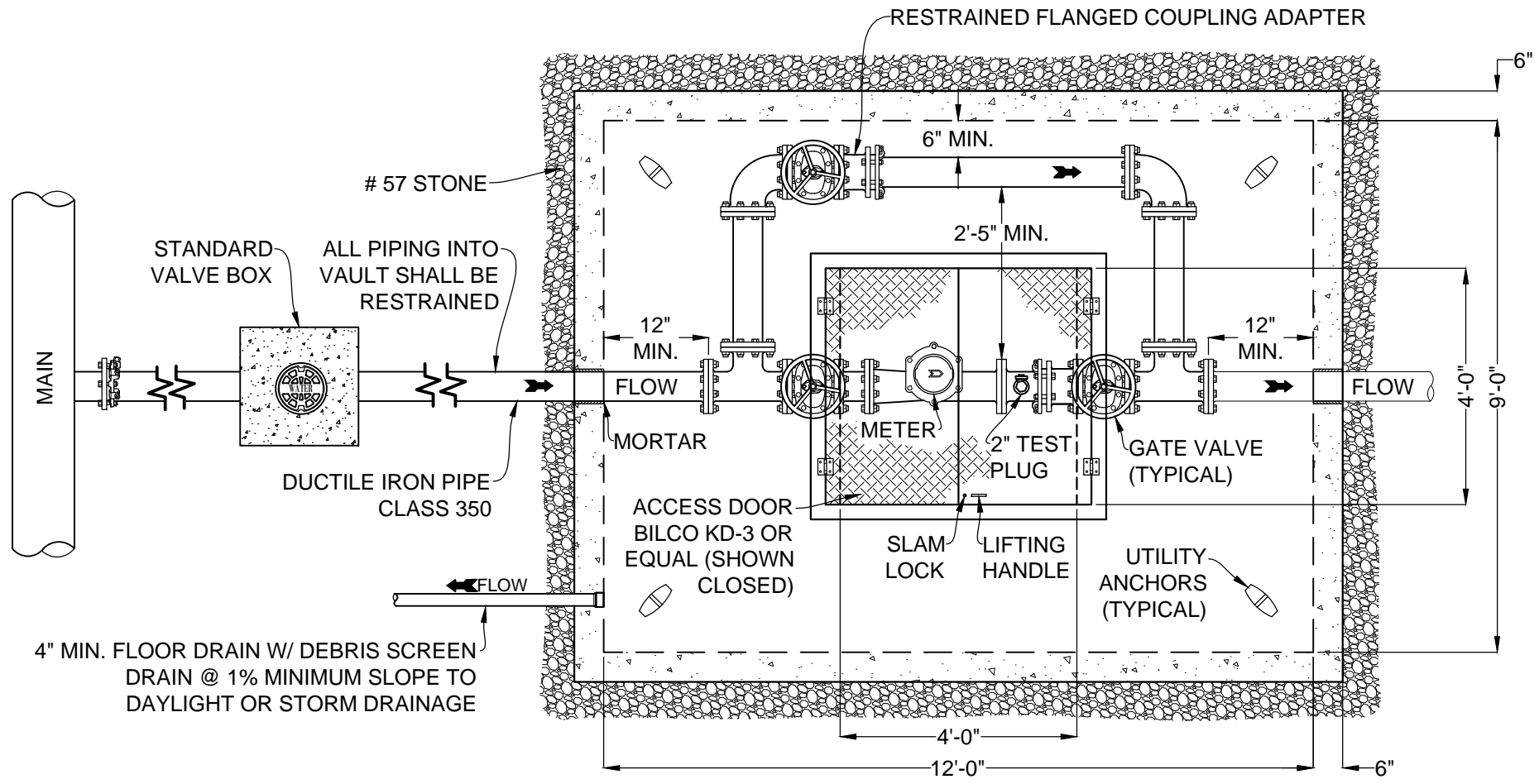
PLAN VIEW
