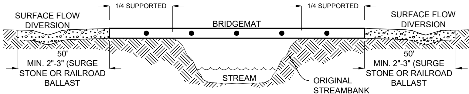
SIDE VIEW
